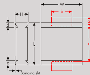
Solder pad recommendation.
